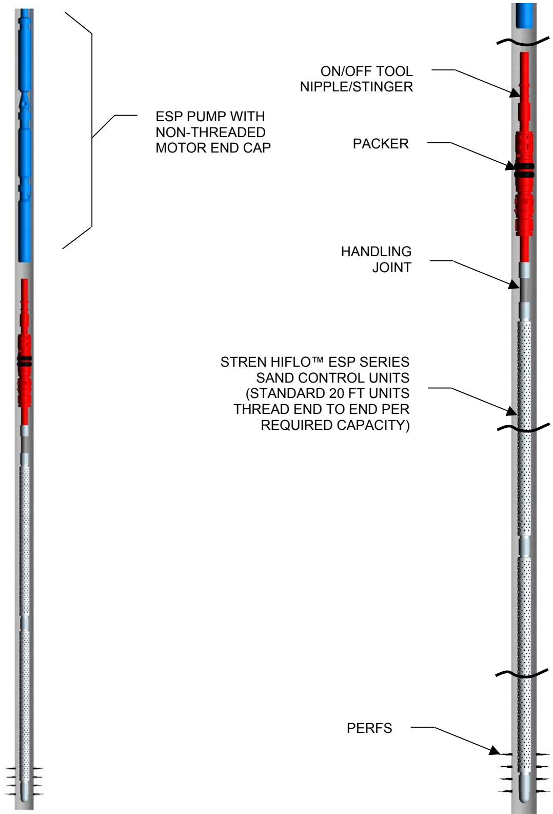
PUMPGARD™ HIFLO ESP SERIES 450 & 550 SAND CONTROL FOR PROTECTING AND EXTENDING ESP PUMP LIFE
